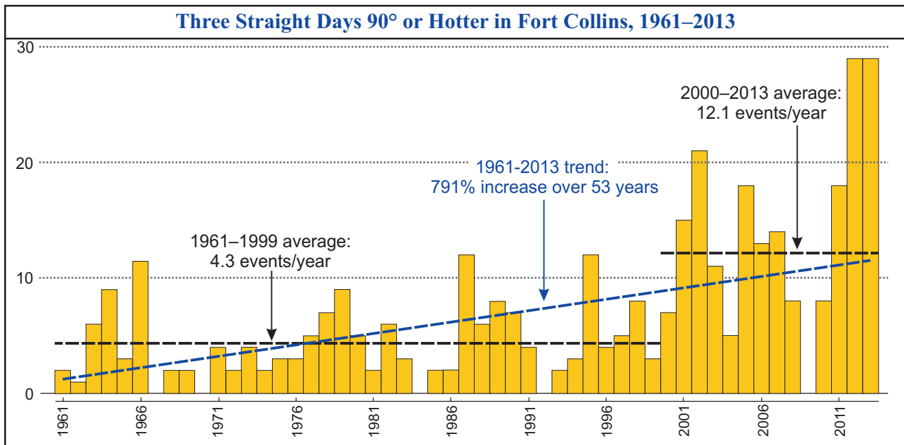
Figure 2. Occurrences per year of three straight days each with maximum temperatures of 90° or hotter; otherwise as in Figure 1. Note that occurrences may overlap, so that, for example, four straight 90° days count as two separate occurrences (see text on this page).
