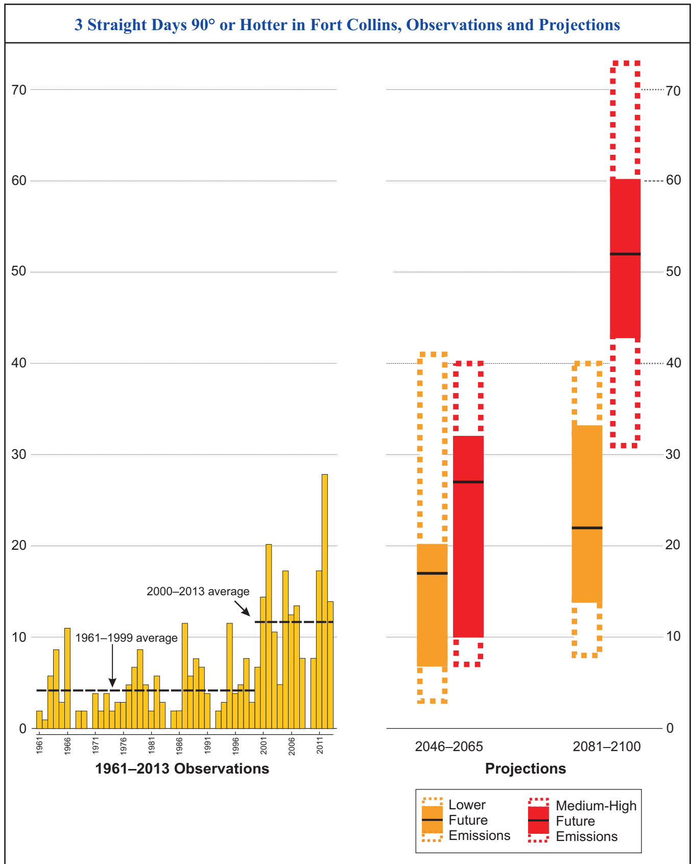
Figure 6. Occurrences per year of three straight days each with maximum temperatures of 90° or hotter; otherwise as in Figure 5. Again, note that occurrences may overlap (see text on page 2). For the values of the projections shown in this figure, see Table 3 on page 13.
