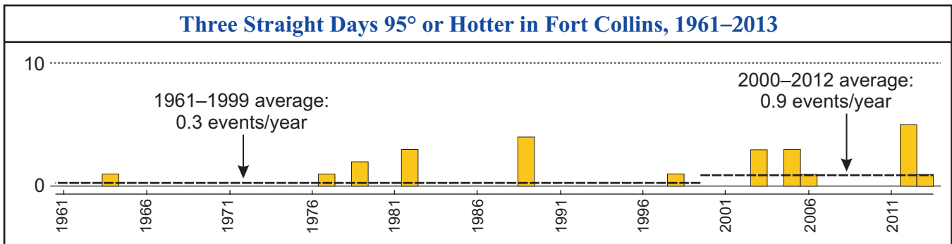
Figure 4. Occurrences per year of three straight days each with maximum temperatures of 95° or hotter. Otherwise, as in Figure 1, except that no linear trend is shown because so many years have no occurrences. Again, note that occurrences may overlap (see text on page 2).
