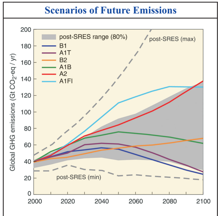
Figure 8. Annual levels of emissions of heat-trapping pollution assumed in selected emissions scenarios, including those cited in this report (B1, or "lower," and A2, or "medium-high"). Dashes indicate the range of newer, replacement ("post-SRES") scenarios now beginning to be used; the gray area represents the middle 80th percentile of their range. Figure from the IPCC.
