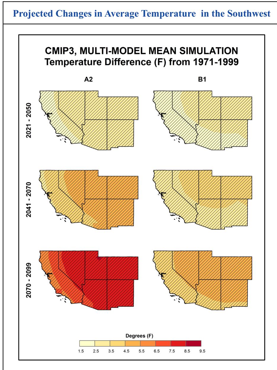
Figure 7. Projected changes in average annual temperatures, showing averages of projections from one model run apiece from 15 downscaled global climate model for emissions scenario A2 (referred to in this report as having medium-high emissions) and from 14 for scenario B1 (referred to here as having lower emissions). Hatching indicates that more than 50% of the simulations show a statistically significant change and that more than 67% agree on the direction of the change. Figure from National Oceanic and Atmospheric Administration. 3
