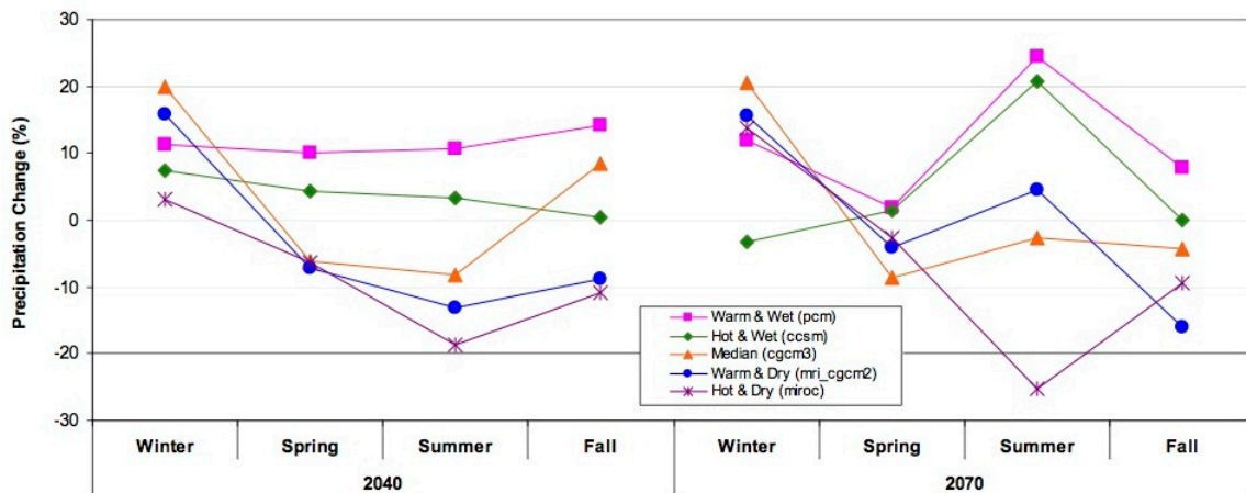
Figure 8. Average seasonal percent change in precipitation for the Front Range of Colorado, projected for mid-century (left; 2035-45) and late-century (right; 2065-75). From Joint Front Range Climate Change Vulnerability Study 2012. Water Research Foundation. 1
