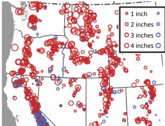
Figure 12. Increases (in blue) and decreases (in red) in April 1 st snow-water equivalent (SWE) over the 1960–2002 period of record, adapted from Mote. 12
