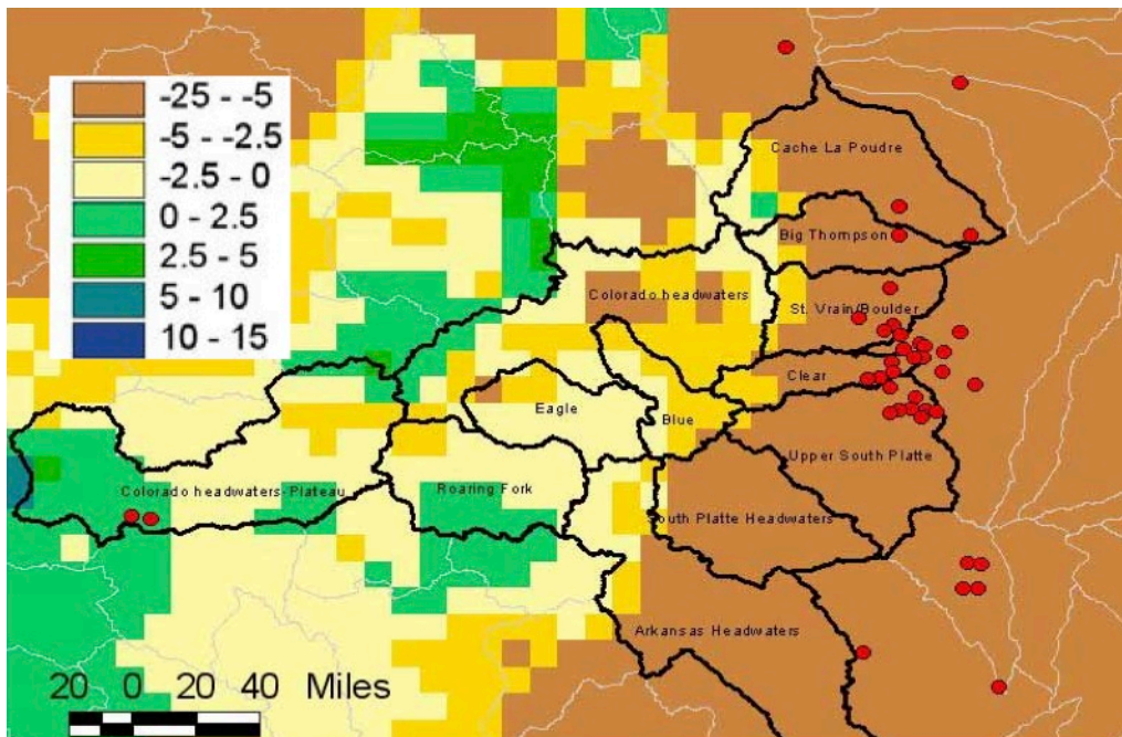
Figure 11. Percent change in total annual average precipitation between the historical period (1950-2000) and the 2070 period (2055-2084) based on the MIROC model. From Joint Front Range Climate Change Vulnerability Study 2012. Water Research Foundation. 1
