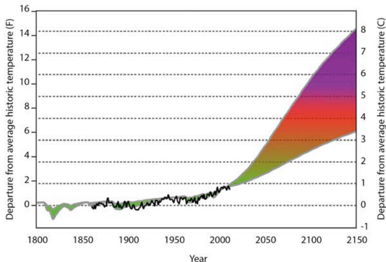
Figure 4. Average global temperatures since 1800, in comparison to projected temperatures through 2150. Data provided by the Environmental Change Institute, University of Oxford. Modeling by Richard Millar consistent with, but not identical to, the projections of the IPCC.
