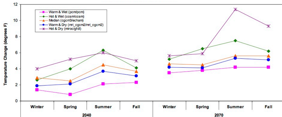
Figure 6. Average temperature change for the Front Range of Colorado, by season, projected for mid-century (left; 2035-45) and late-century (right; 2065-75). From Joint Front Range Climate Change Vulnerability Study 2012. Water Research Foundation. 1
