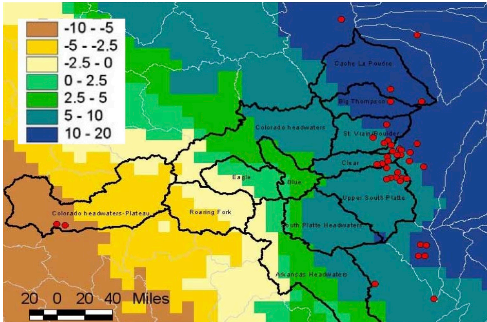
Figure 10. Percent change in total annual average precipitation between the historical period (1950-2000) and the 2070 period (2055-2084) based on the ccsm model. From Joint Front Range Climate Change Vulnerability Study 2012. Water Research Foundation. 1
