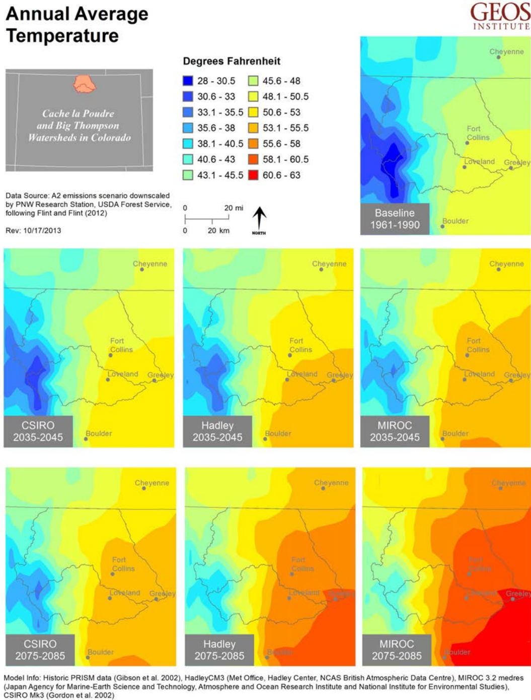
Figure 7. Average annual temperature across Cache La Poudre and Colorado-Big Thompson Watersheds for the historic period (1961-90) and two future time periods (2035-45 and 2075-85), projected using three different climate models (CSIRO, HadCM, and MIROC) and the A2 emissions scenario.
